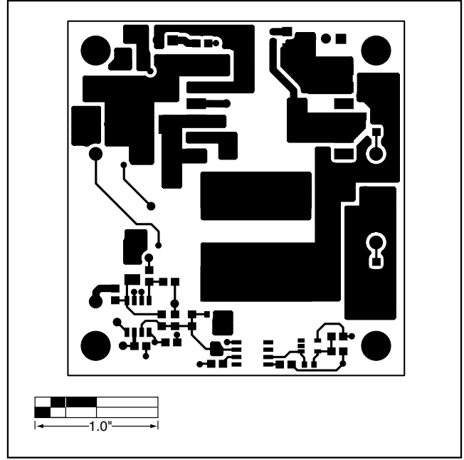
Figure 6. MAX5015 EV Kit PCB Layout—Component Side
